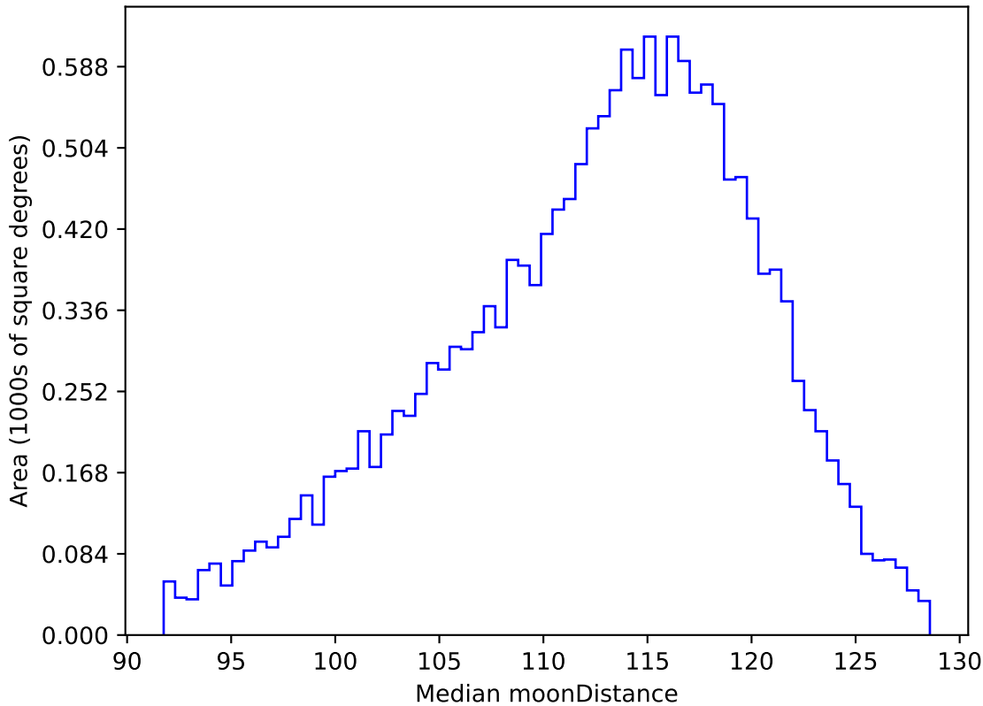
weather_cloudso36v3.4_10yrs WFD r band: Median moonDistance
