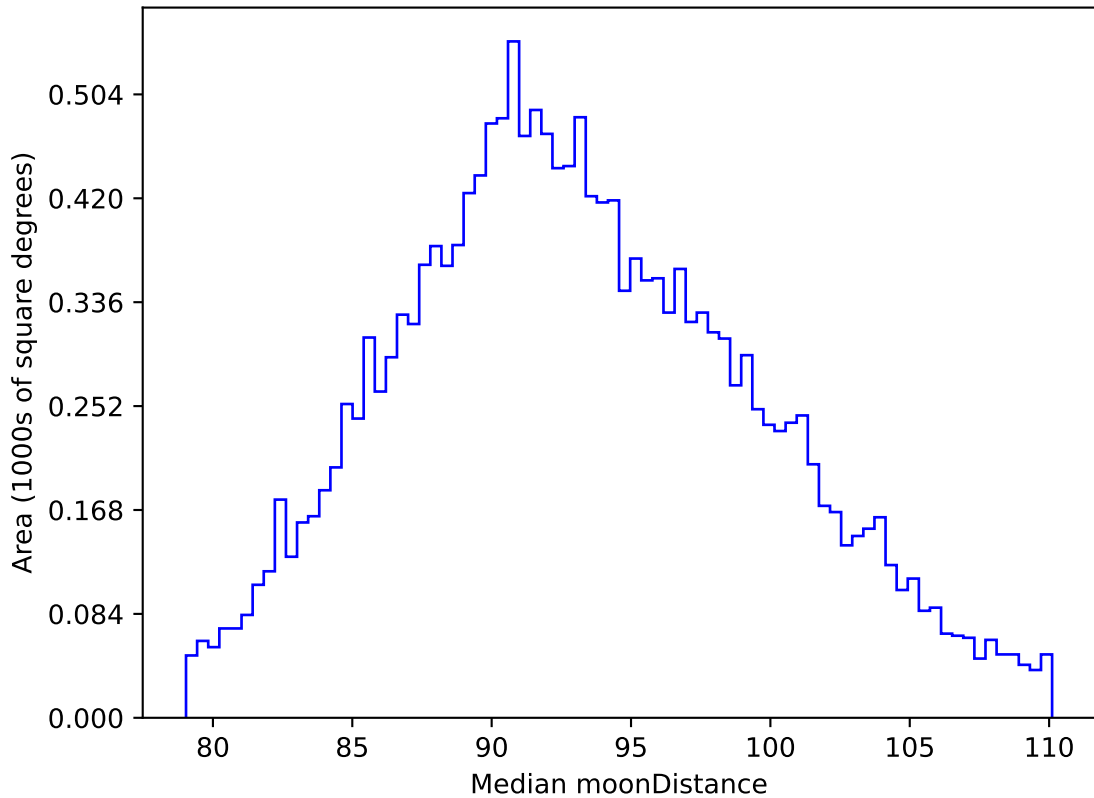
weather_cloudso36v3.4_10yrs WFD i band: Median moonDistance
