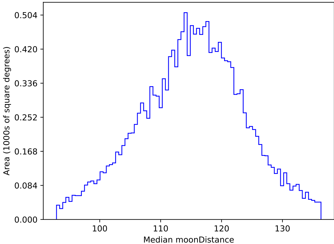
weather_cloudso36v3.4_10yrs WFD g band: Median moonDistance
