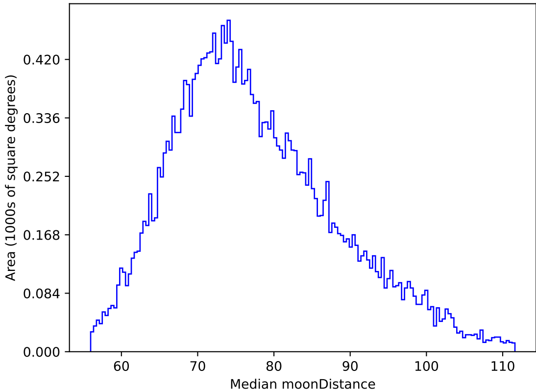
weather_cloudso36v3.4_10yrs All sky z band: Median moonDistance
