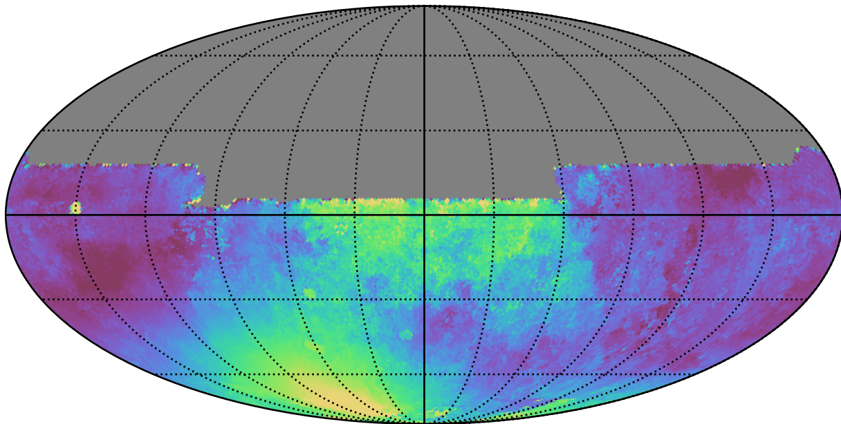
weather_cloudso36v3.4_10yrs All sky y band: Median moonDistance
