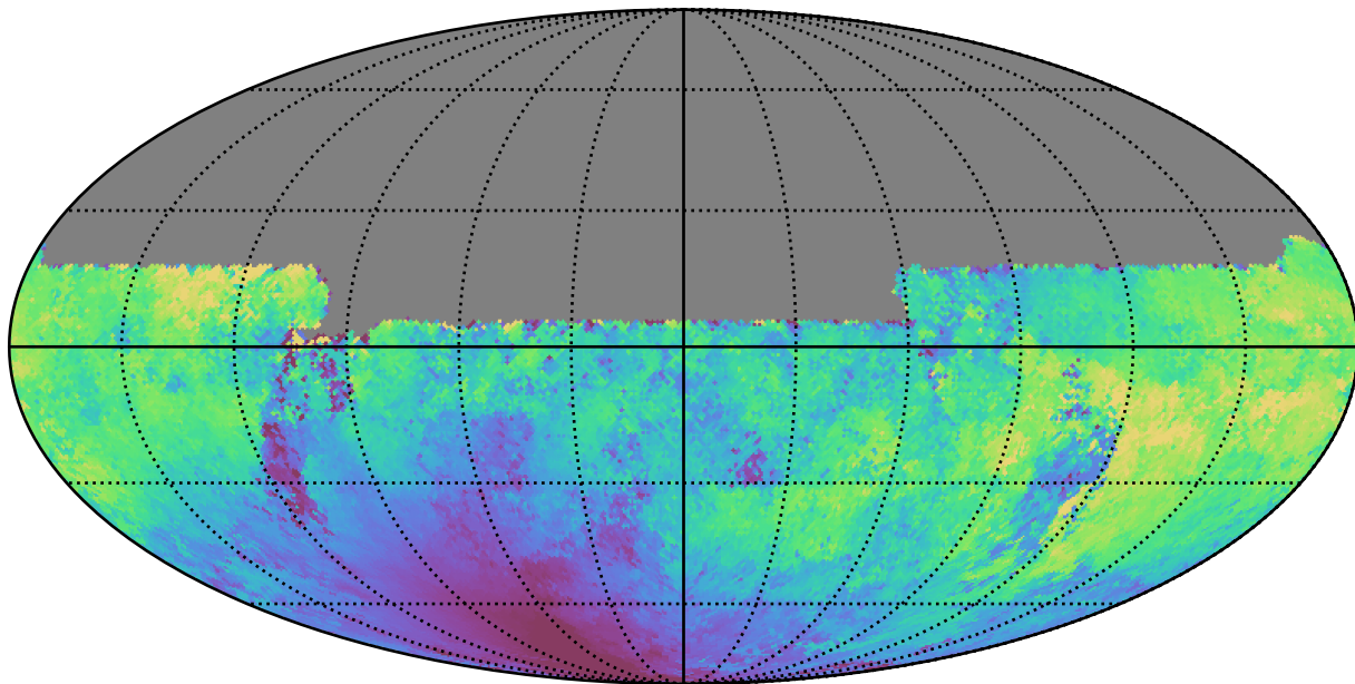
weather_cloudso36v3.4_10yrs All sky u band: Median moonDistance
