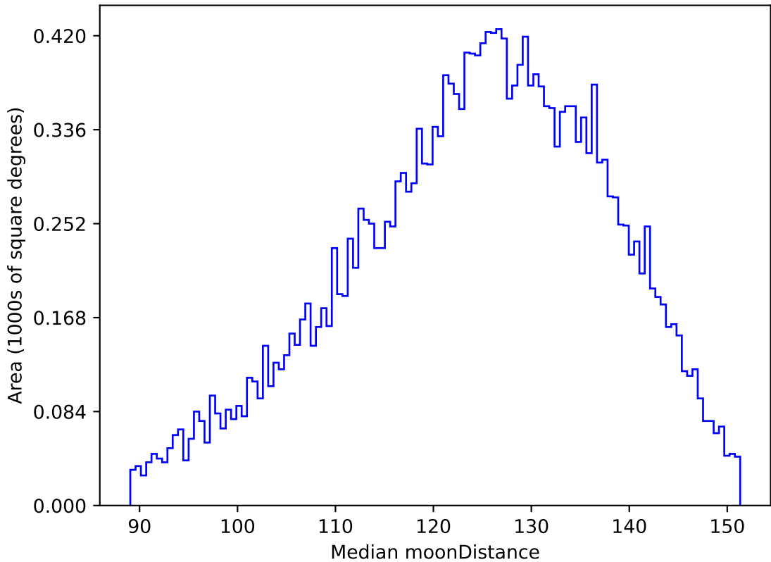
weather_cloudso36v3.4_10yrs All sky u band: Median moonDistance
