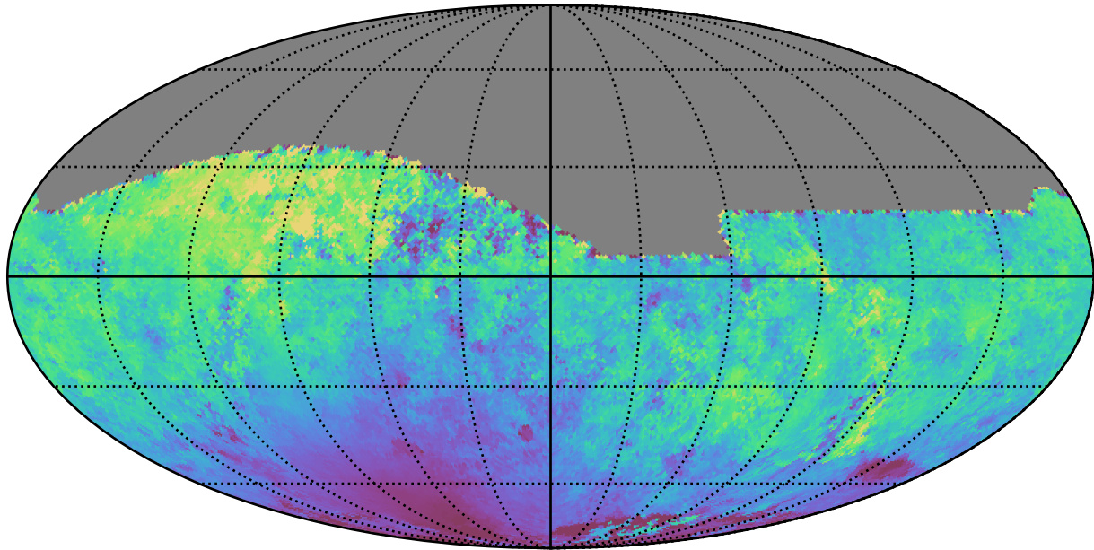
weather_cloudso36v3.4_10yrs All sky r band: Median moonDistance
