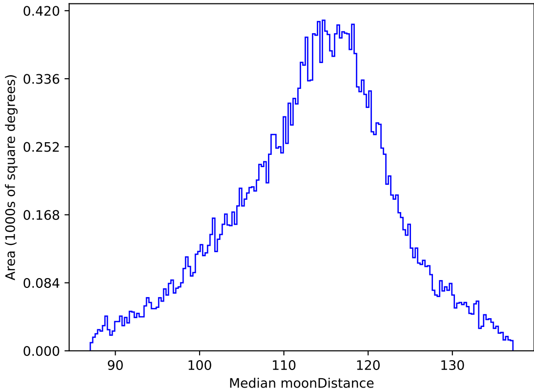
weather_cloudso36v3.4_10yrs All sky r band: Median moonDistance
