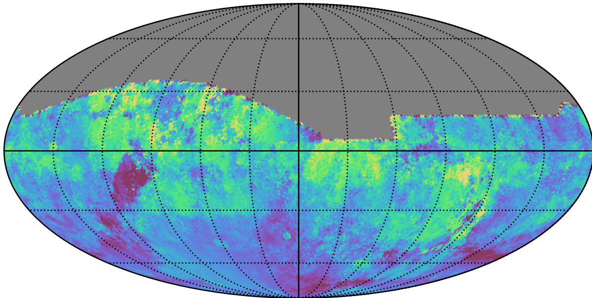
weather_cloudso36v3.4_10yrs All sky i band: Median moonDistance
