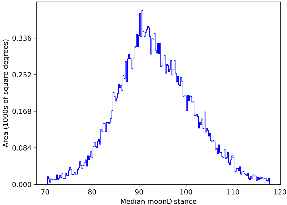
weather_cloudso36v3.4_10yrs All sky i band: Median moonDistance
