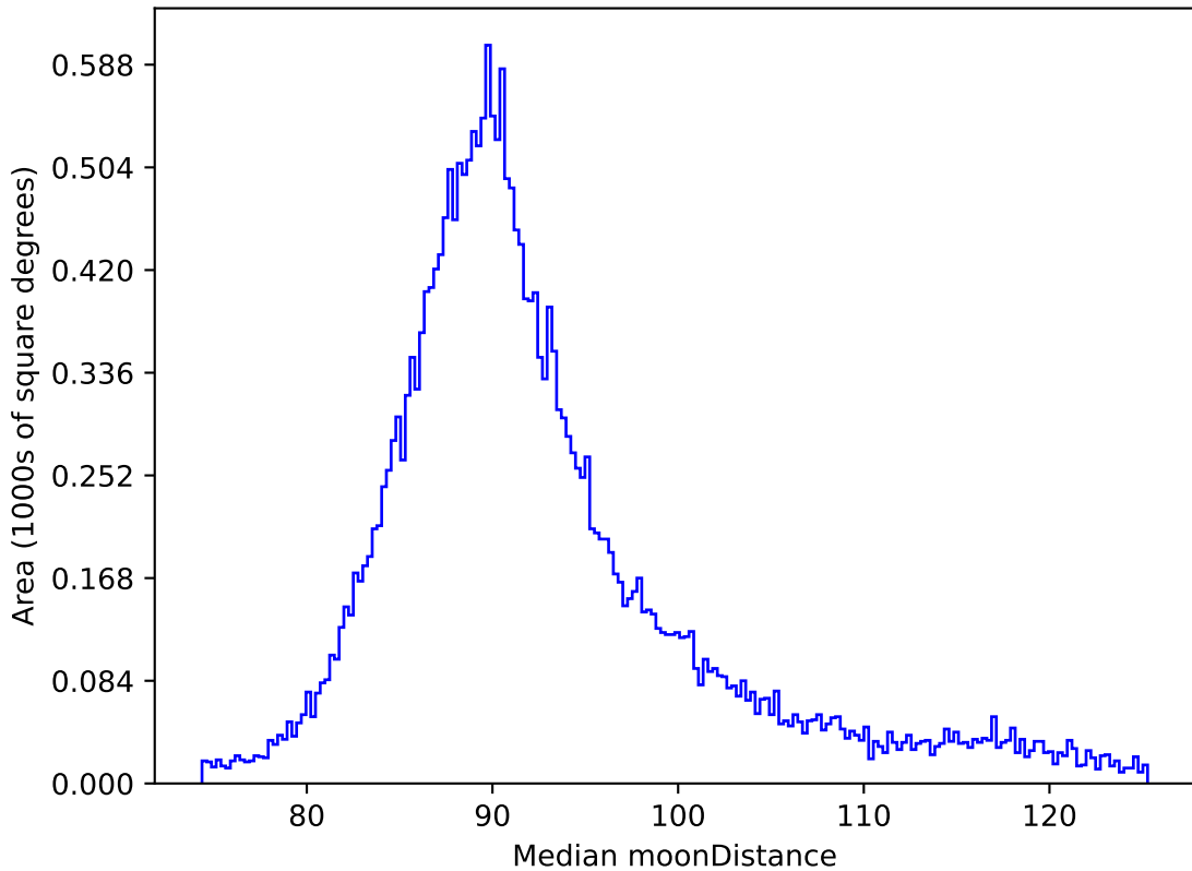
weather_cloudso36v3.4_10yrs All sky all bands: Median moonDistance
