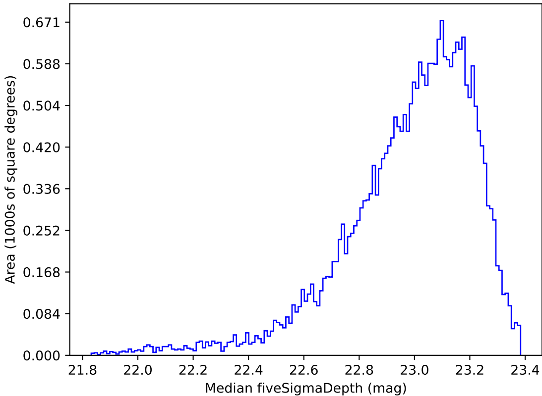
weather_cloudso36v3.4_10yrs Yr 1 z band: Median fiveSigmaDepth
