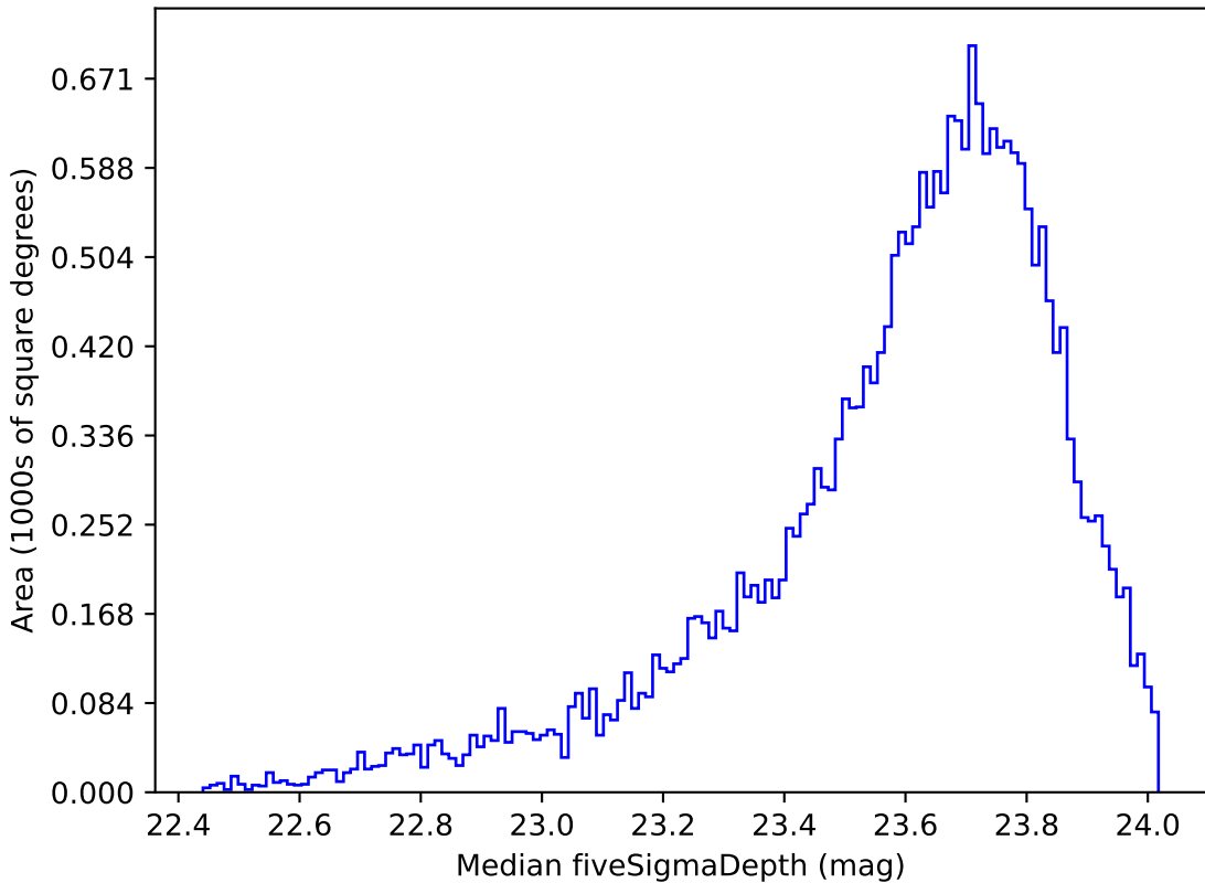
weather_cloudso36v3.4_10yrs Yr 1 i band: Median fiveSigmaDepth
