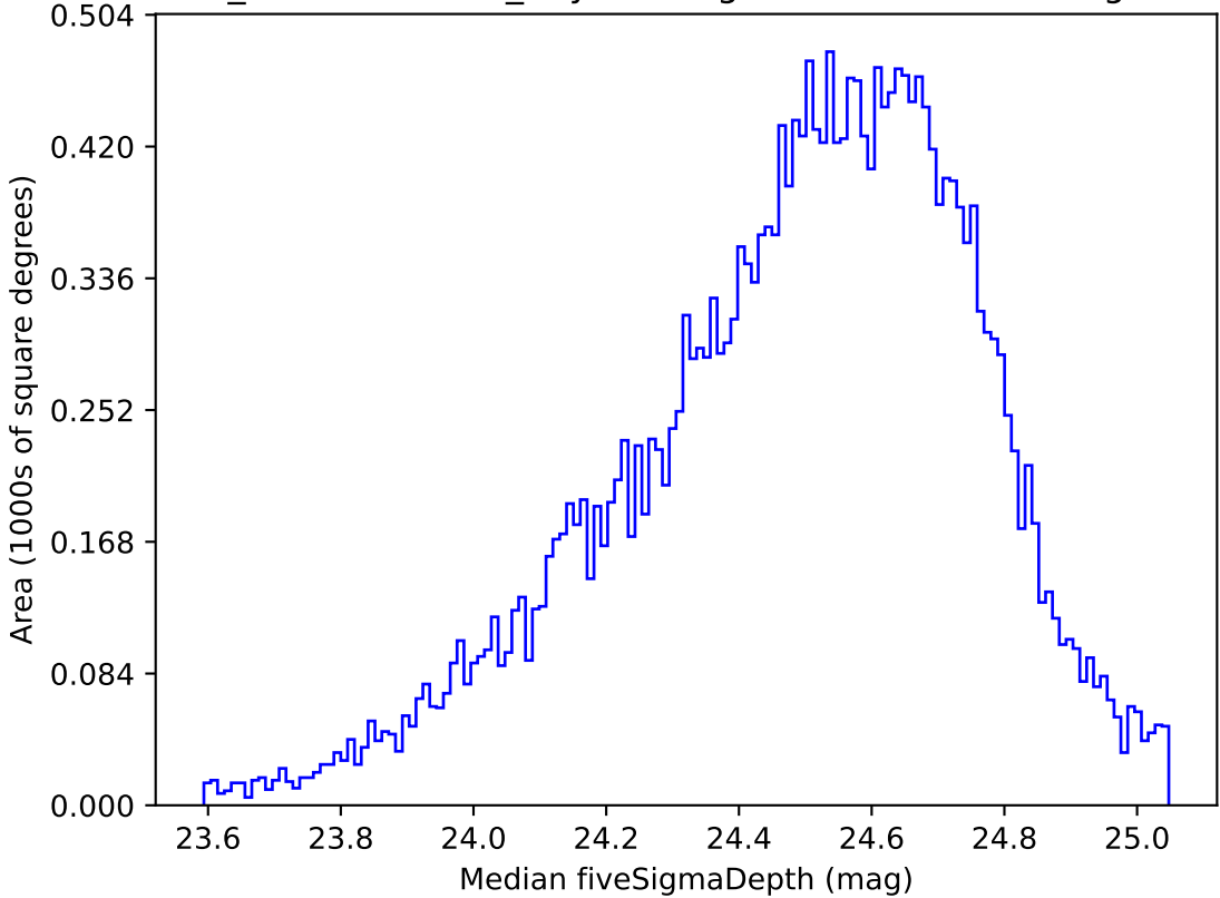
weather_cloudso36v3.4_10yrs Yr 1 g band: Median fiveSigmaDepth
