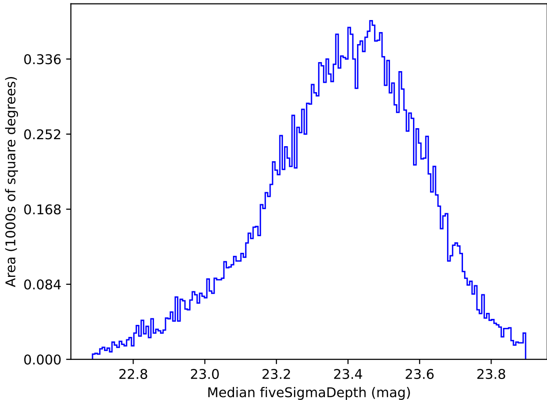
weather_cloudso36v3.4_10yrs Yr 1 all bands: Median fiveSigmaDepth
