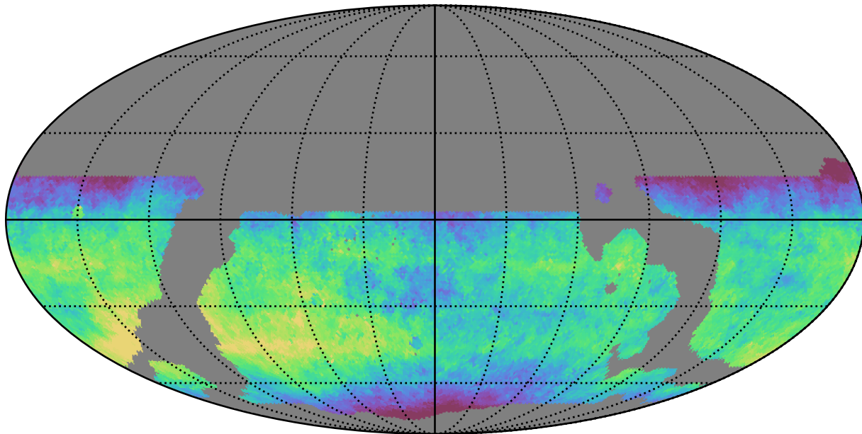
weather_cloudso36v3.4_10yrs WFD z band: Median fiveSigmaDepth
