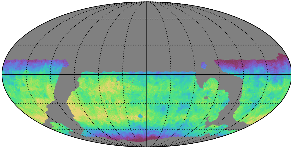
weather_cloudso36v3.4_10yrs WFD y band: Median fiveSigmaDepth
