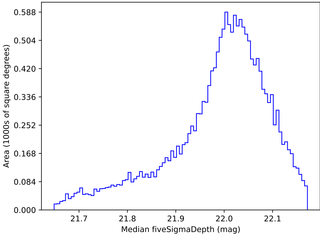
weather_cloudso36v3.4_10yrs WFD y band: Median fiveSigmaDepth
