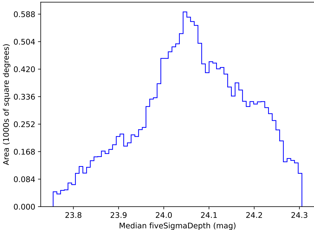
weather_cloudso36v3.4_10yrs WFD r band: Median fiveSigmaDepth
