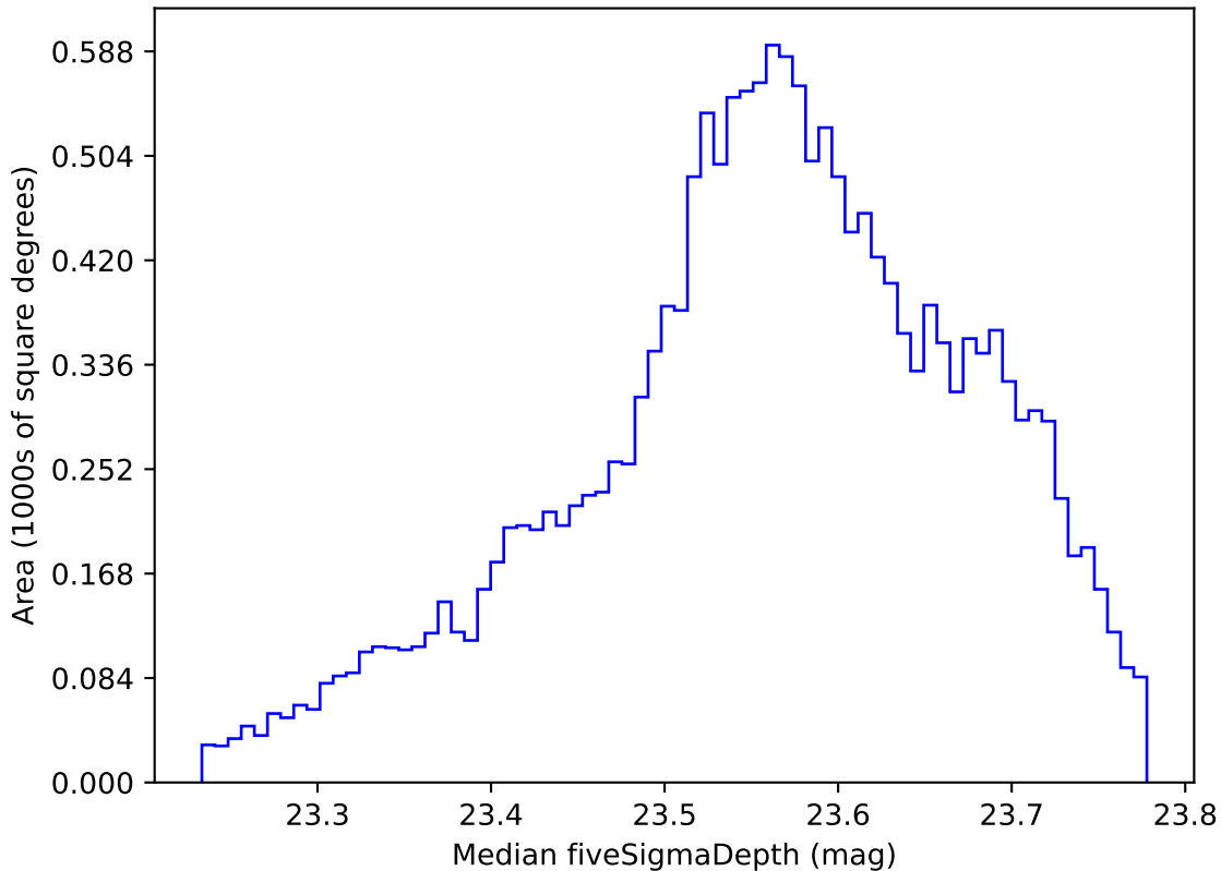
weather_cloudso36v3.4_10yrs WFD i band: Median fiveSigmaDepth
