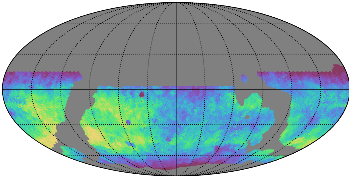
weather_cloudso36v3.4_10yrs WFD g band: Median fiveSigmaDepth
