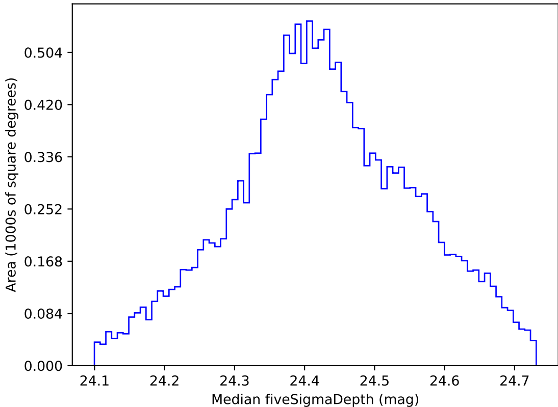
weather_cloudso36v3.4_10yrs WFD g band: Median fiveSigmaDepth
