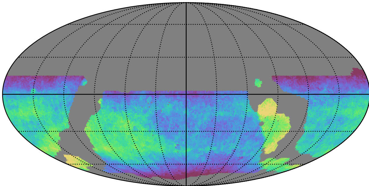
weather_cloudso36v3.4_10yrs WFD all bands: Median fiveSigmaDepth
