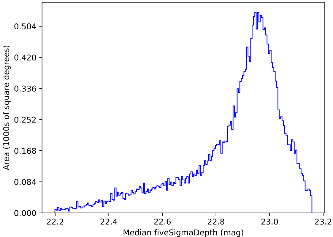
weather_cloudso36v3.4_10yrs All sky z band: Median fiveSigmaDepth
