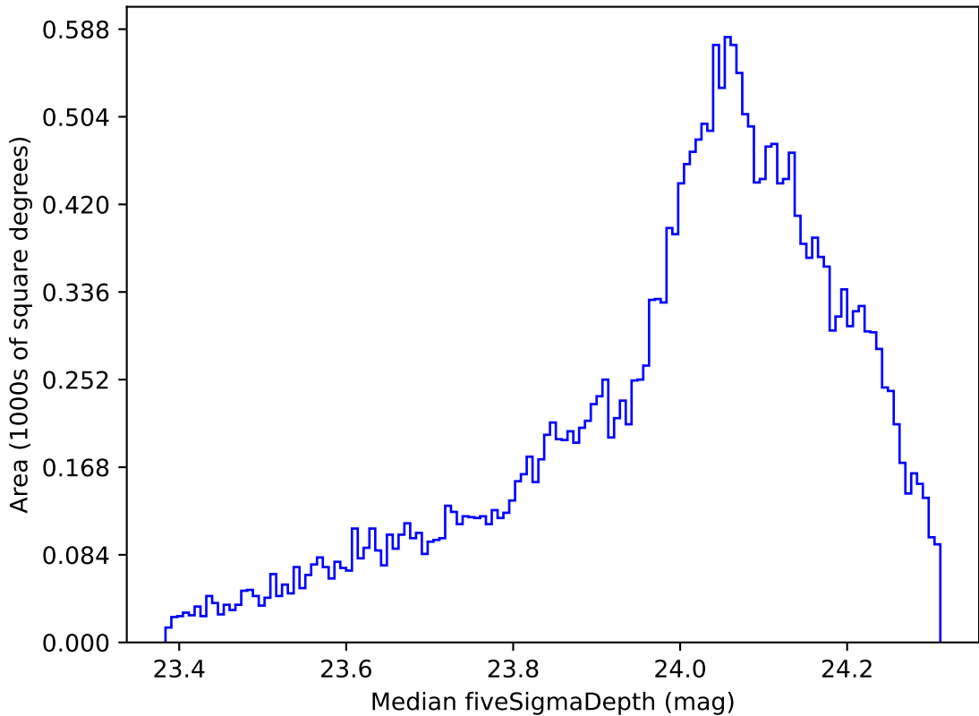
weather_cloudso36v3.4_10yrs All sky r band: Median fiveSigmaDepth
