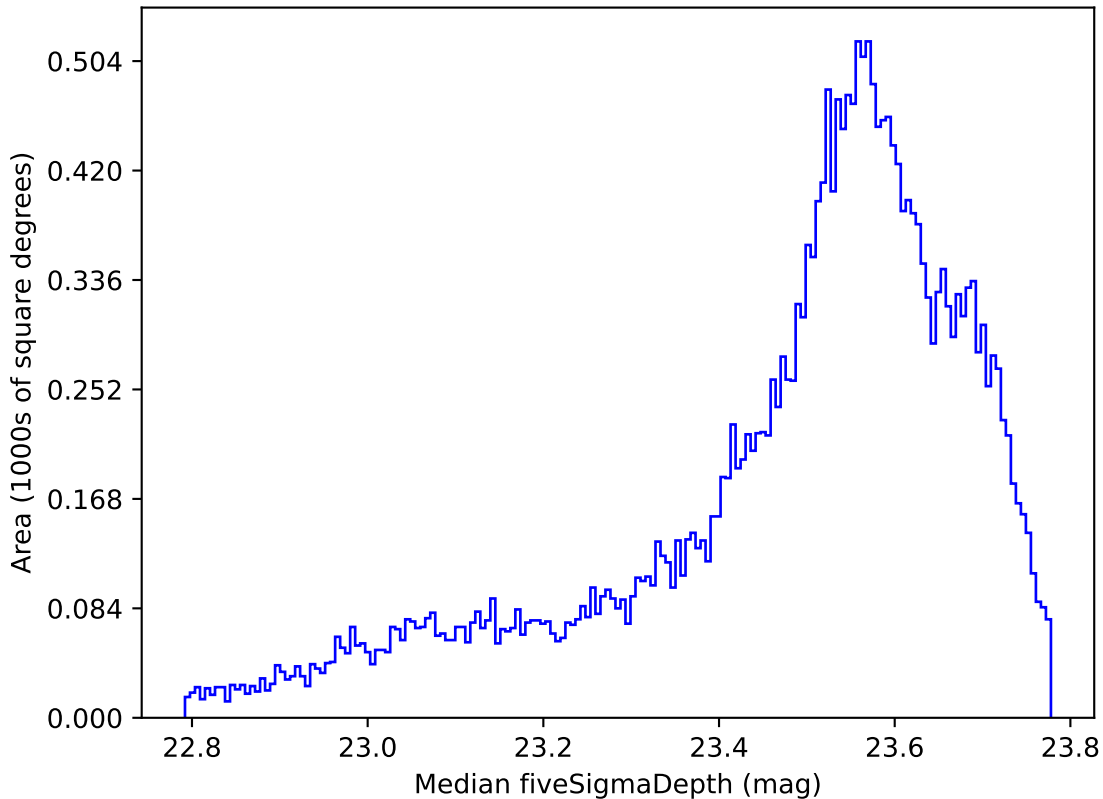
weather_cloudso36v3.4_10yrs All sky i band: Median fiveSigmaDepth
