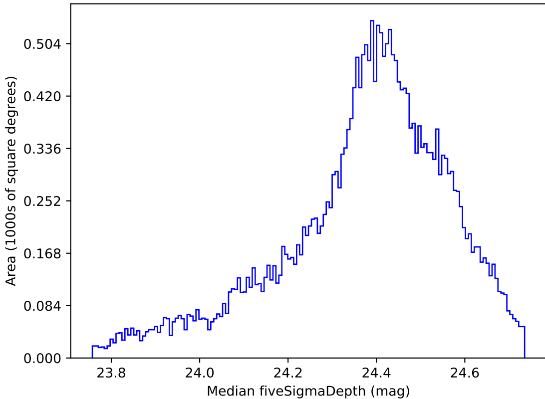
weather_cloudso36v3.4_10yrs All sky g band: Median fiveSigmaDepth
