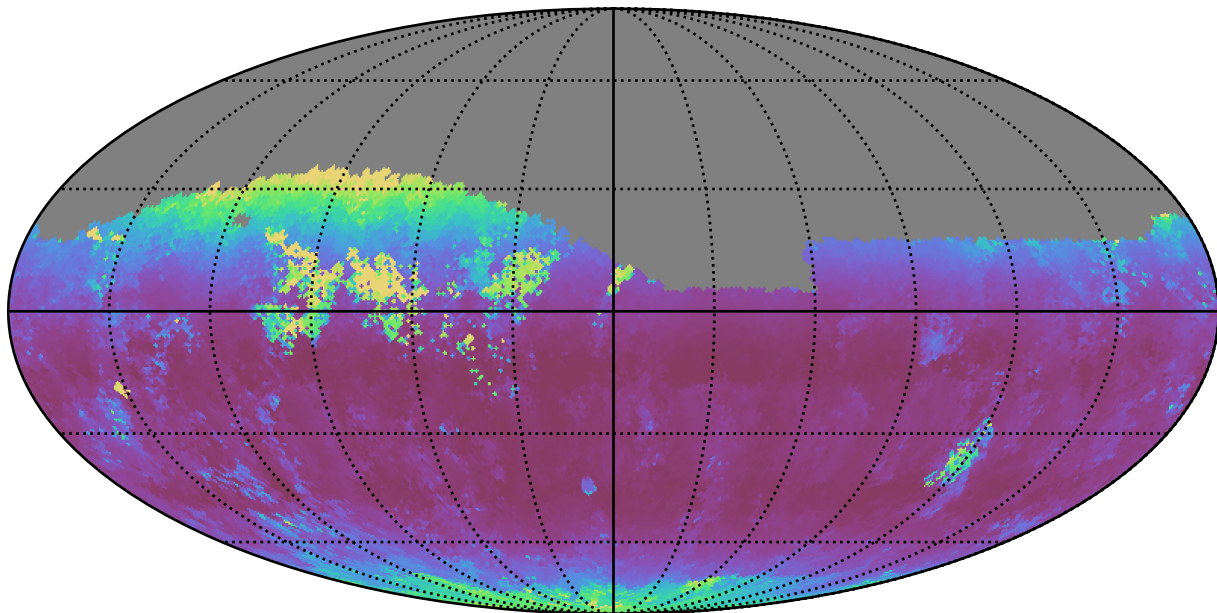
weather_cloudso36v3.4_10yrs Yr 1 z band: Median airmass
