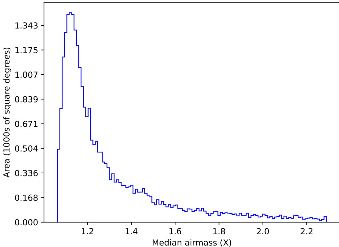
weather_cloudso36v3.4_10yrs Yr 1 z band: Median airmass
