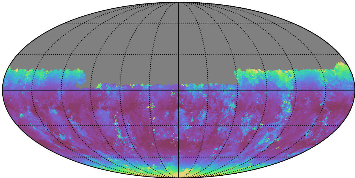
weather_cloudso36v3.4_10yrs Yr 1 u band: Median airmass
