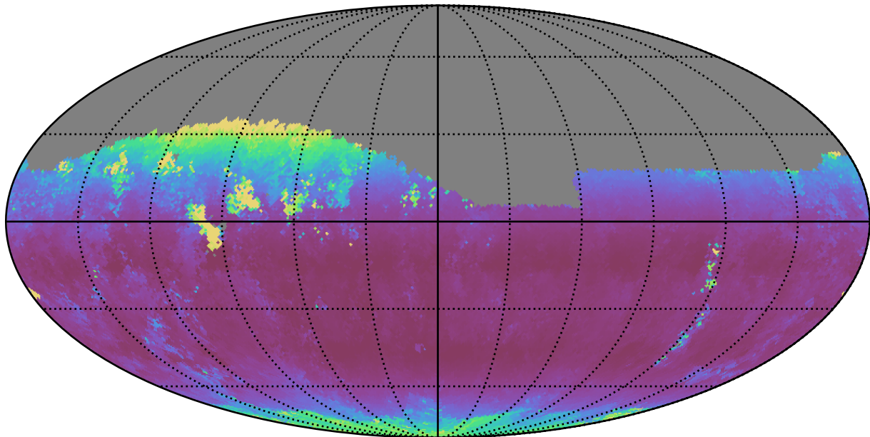
weather_cloudso36v3.4_10yrs Yr 1 i band: Median airmass
