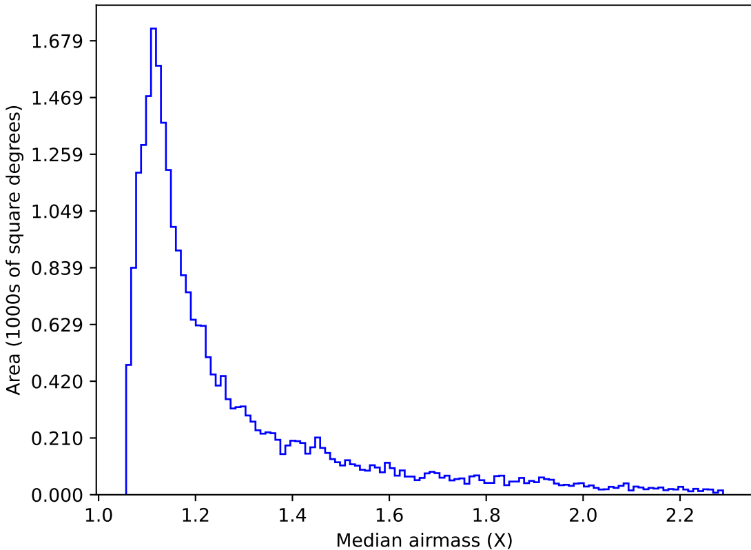
weather_cloudso36v3.4_10yrs Yr 1 i band: Median airmass
