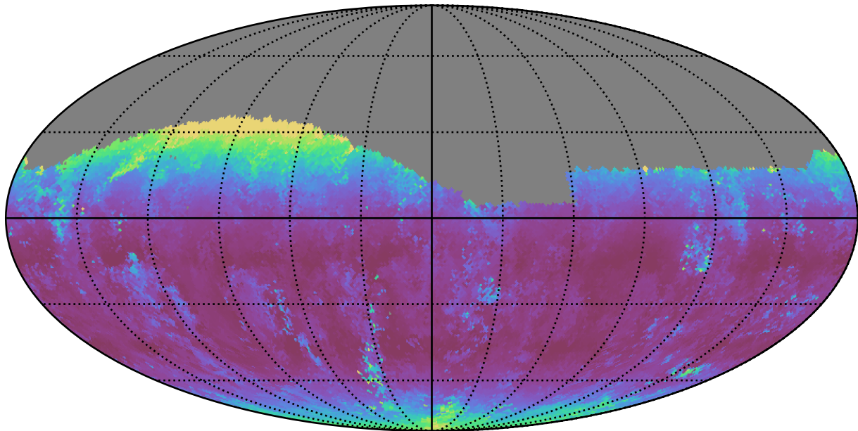
weather_cloudso36v3.4_10yrs Yr 1 g band: Median airmass
