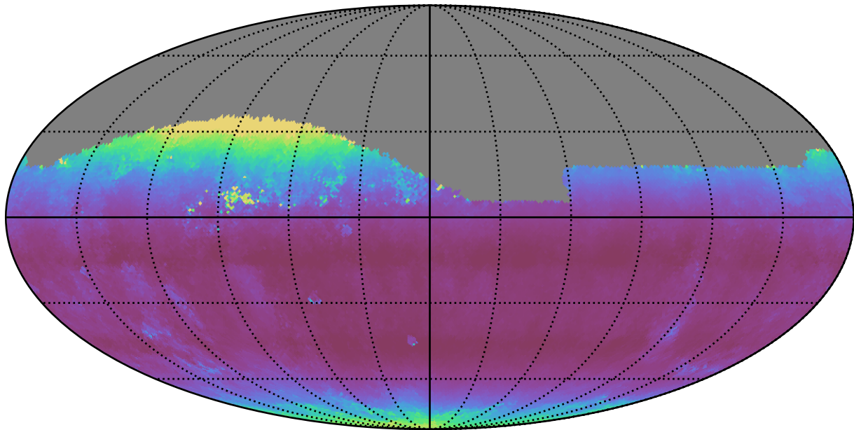
weather_cloudso36v3.4_10yrs Yr 1 all bands: Median airmass
