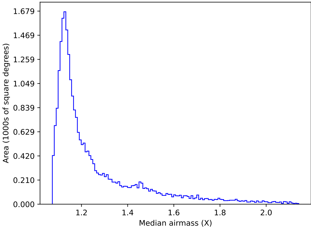
weather_cloudso36v3.4_10yrs Yr 1 all bands: Median airmass
