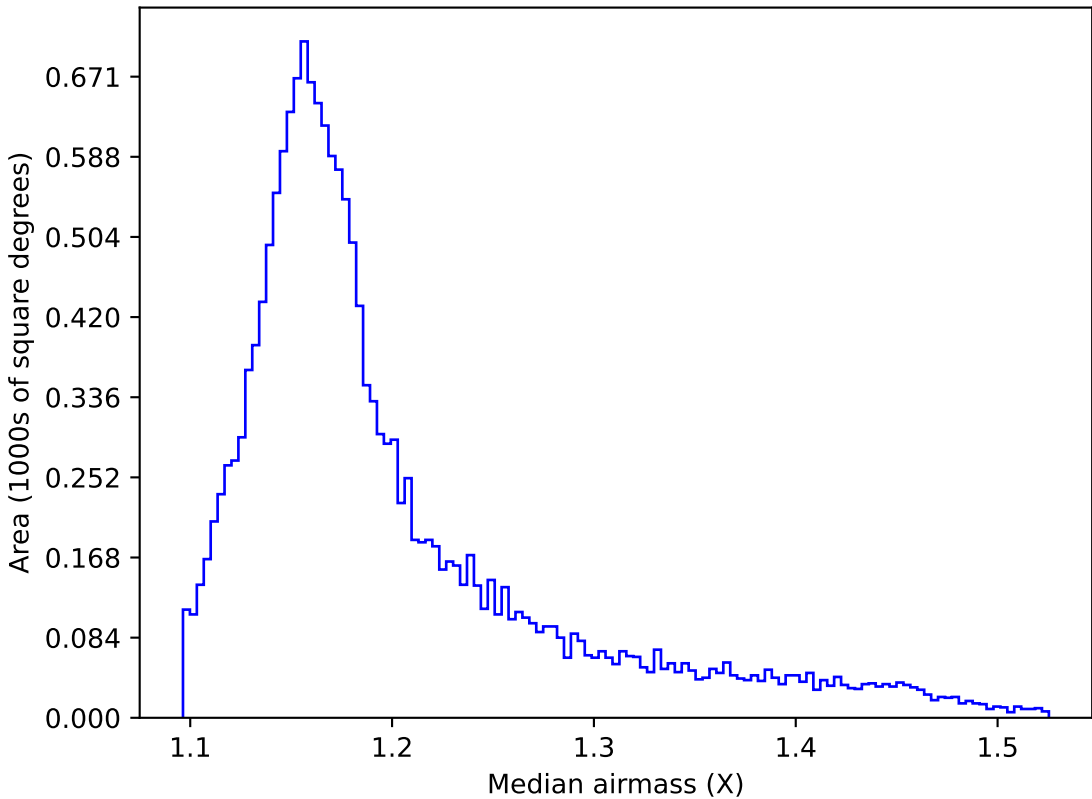
weather_cloudso36v3.4_10yrs WFD z band: Median airmass
