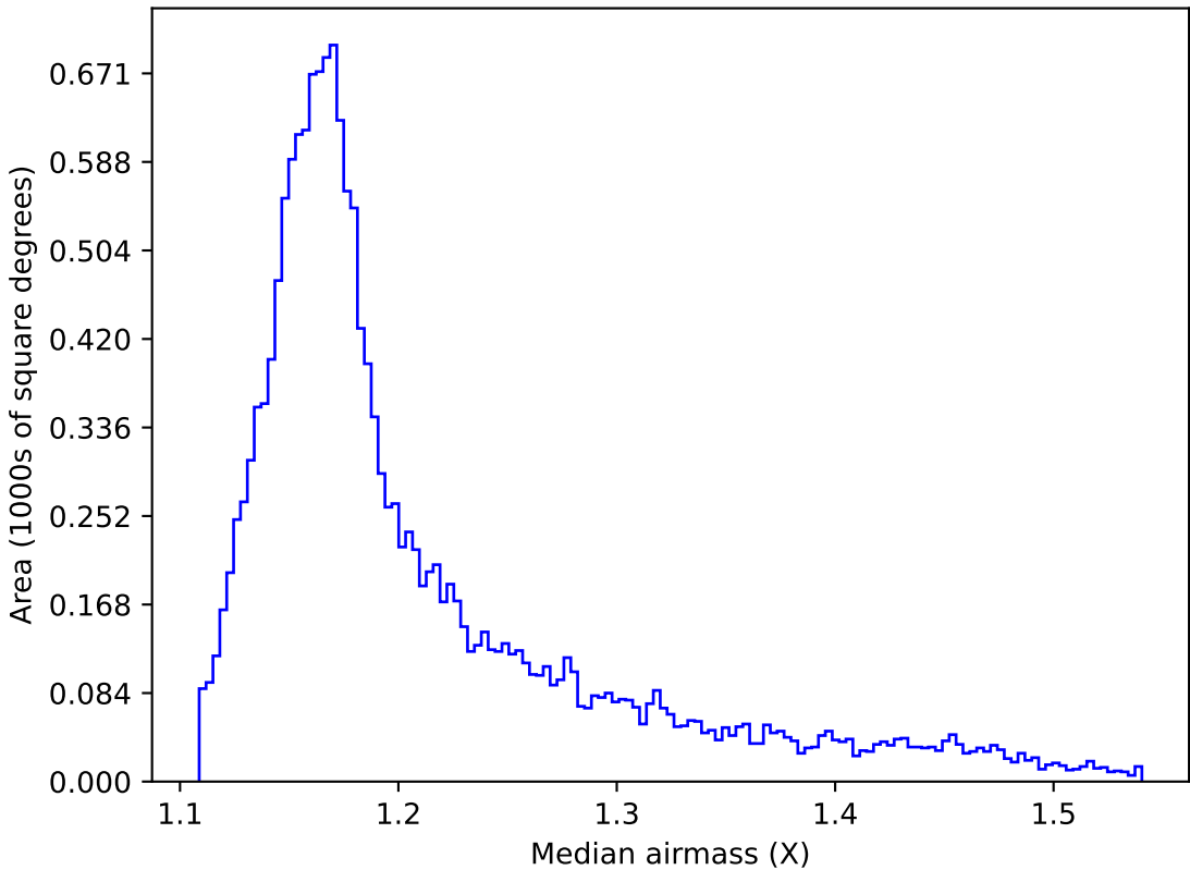
weather_cloudso36v3.4_10yrs WFD y band: Median airmass
