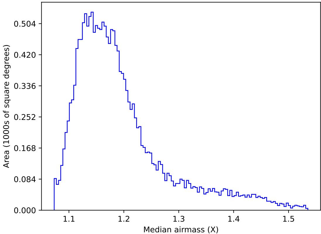
weather_cloudso36v3.4_10yrs WFD u band: Median airmass
