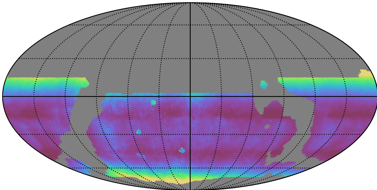
weather_cloudso36v3.4_10yrs WFD r band: Median airmass
