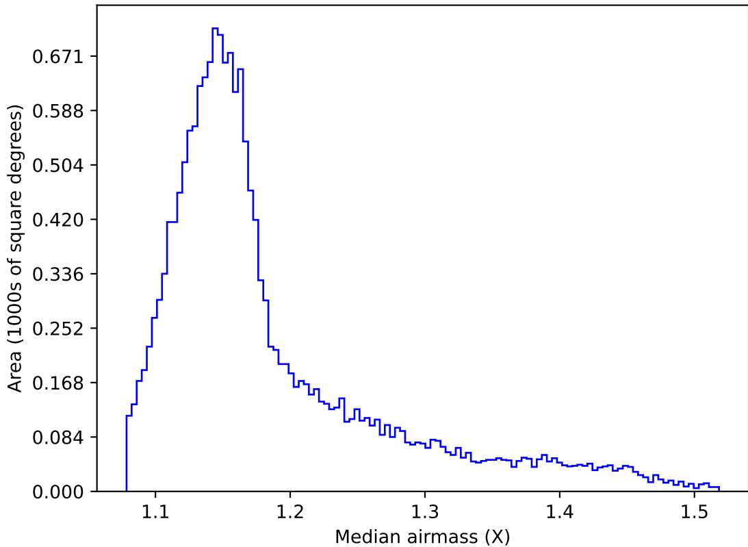
weather_cloudso36v3.4_10yrs WFD r band: Median airmass
