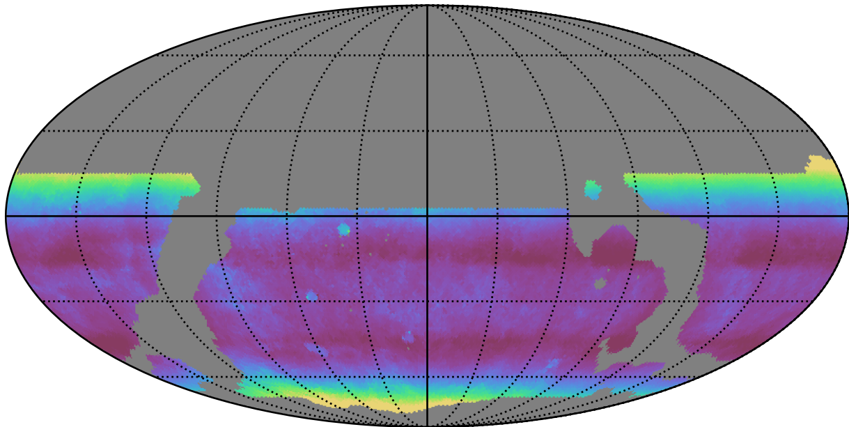
weather_cloudso36v3.4_10yrs WFD i band: Median airmass
