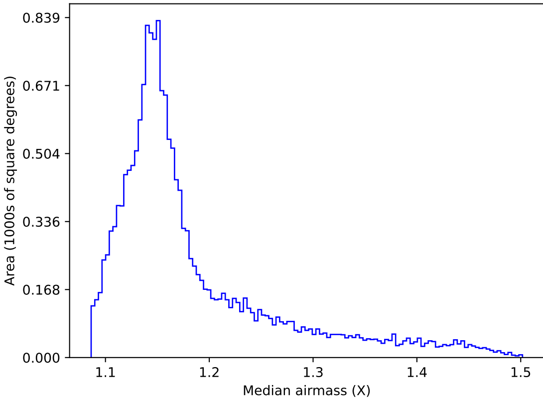
weather_cloudso36v3.4_10yrs WFD i band: Median airmass
