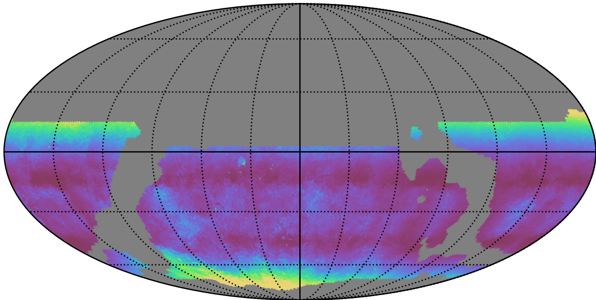
weather_cloudso36v3.4_10yrs WFD g band: Median airmass
