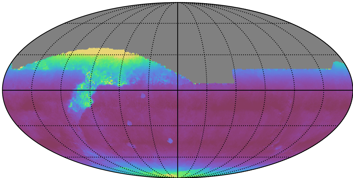
weather_cloudso36v3.4_10yrs All sky z band: Median airmass
