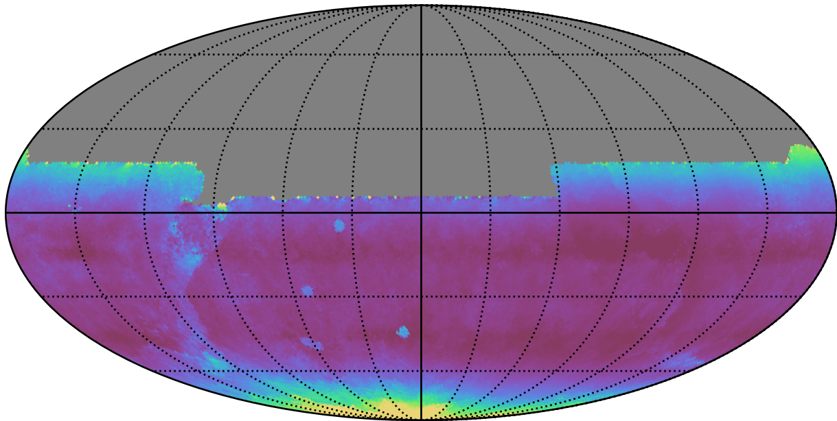
weather_cloudso36v3.4_10yrs All sky y band: Median airmass
