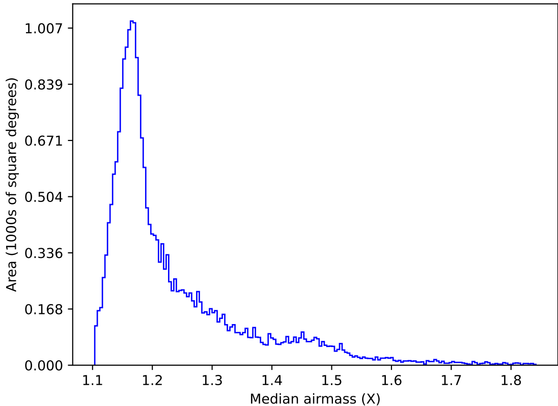
weather_cloudso36v3.4_10yrs All sky y band: Median airmass
