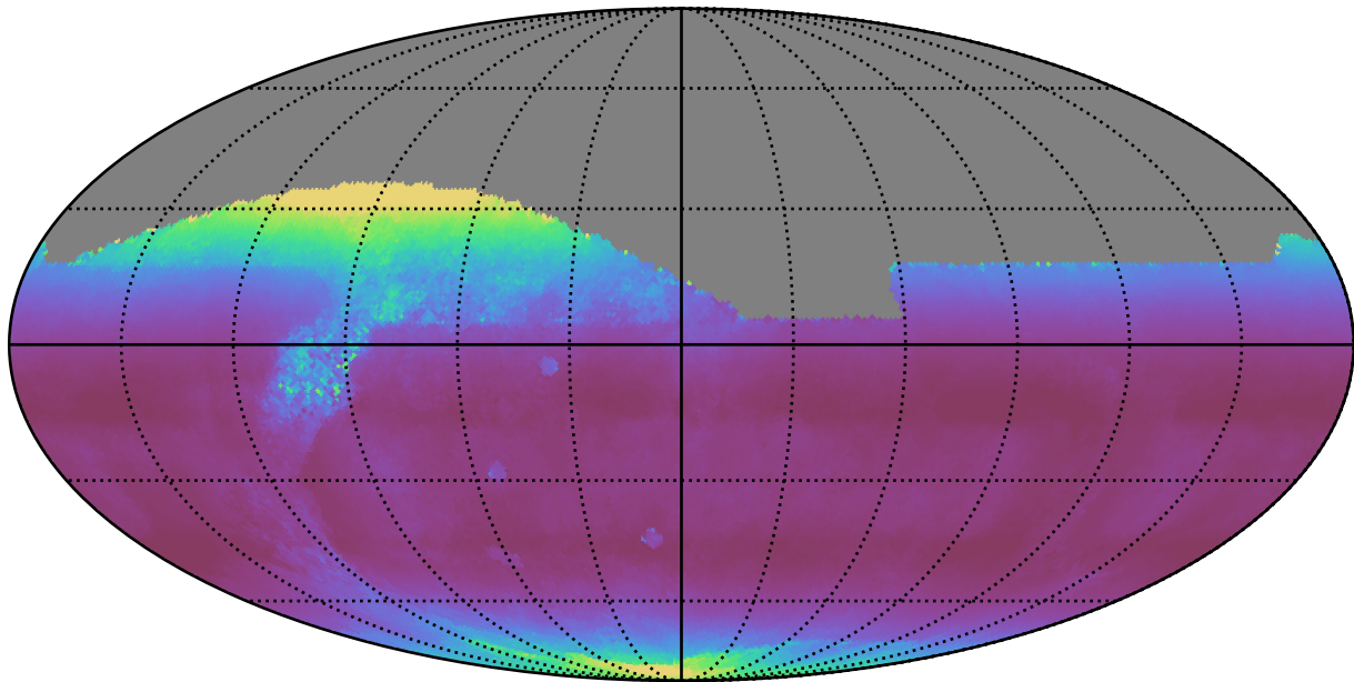
weather_cloudso36v3.4_10yrs All sky r band: Median airmass
