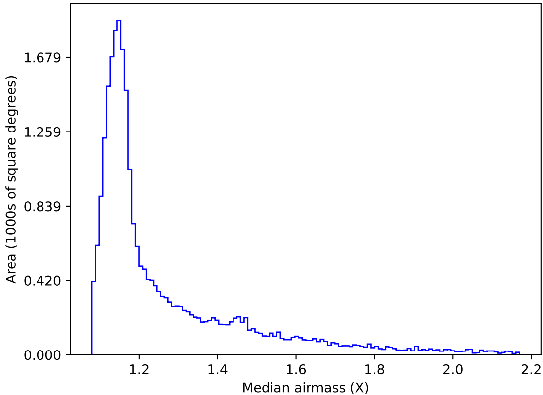
weather_cloudso36v3.4_10yrs All sky r band: Median airmass
