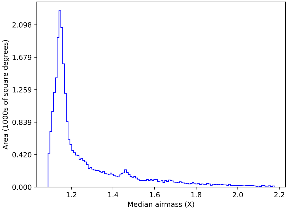
weather_cloudso36v3.4_10yrs All sky i band: Median airmass
